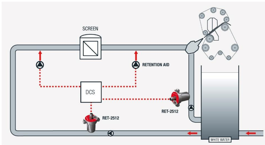
Figure 3: Schematic process diagram of retention aid control with BTG's optical consistency transmitter RET-2512
